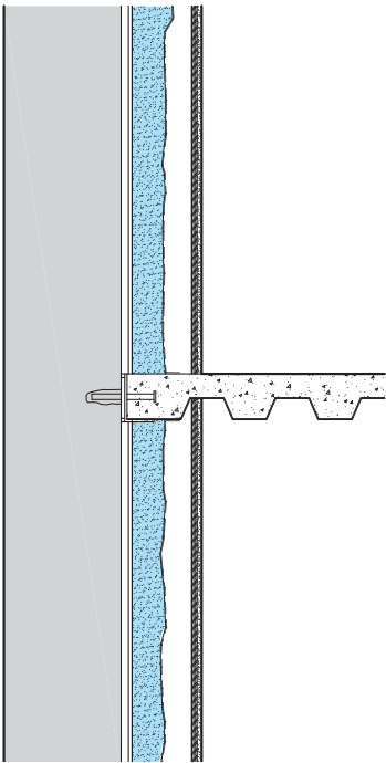
As-Built Condition
