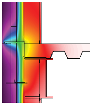
Traditional brick shelf angle
