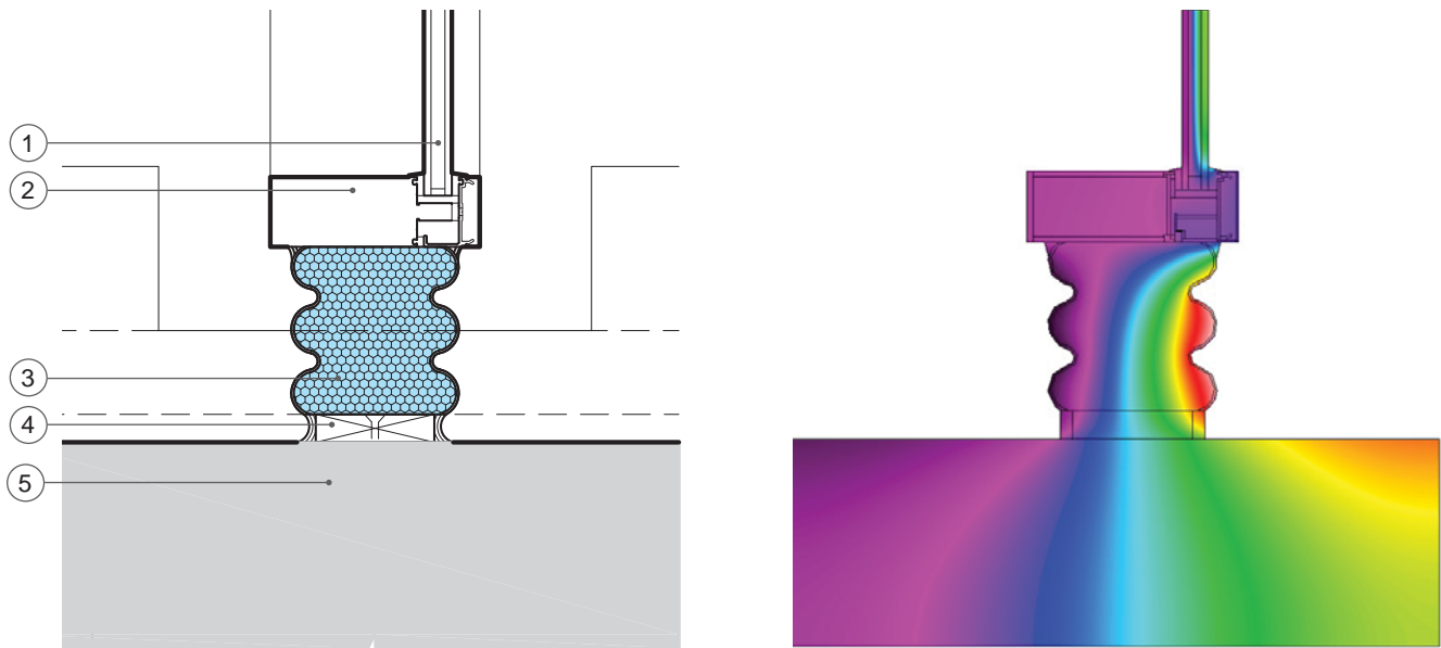
As-Built Condition
