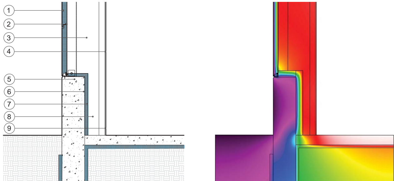
R-8.59 (wall), R-14.21 (floor) (+109% wall, +30.6% floor)
