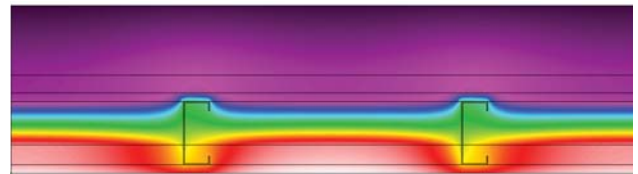
Studs directly attached to existing wall
