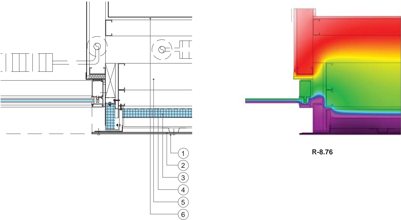
As-Built Condition
