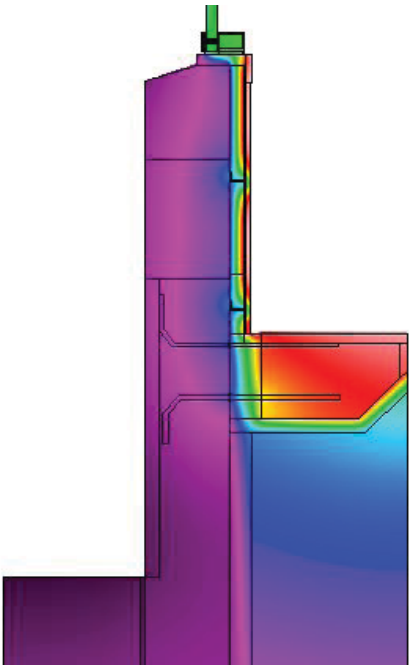
R-6.1 (wall), R-5.85 (floor) (+5% wall, +82.8% floor)
