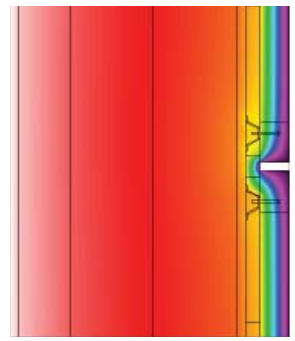
Metal Panel w/ Insulated Joints
