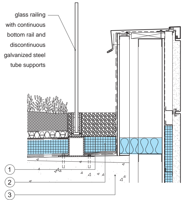
As-Built Condition
