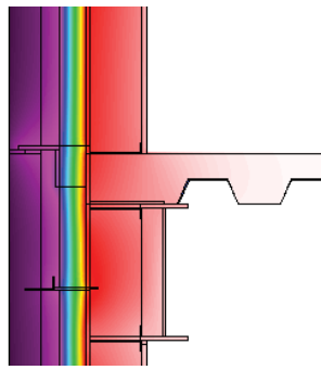
Thermally broken brick shelf angle
