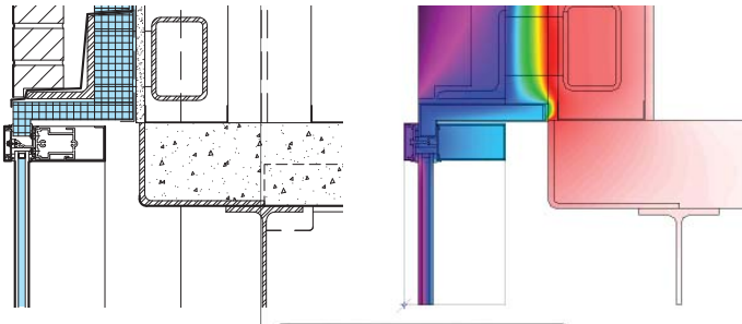
Section Detail
