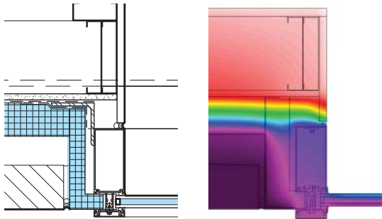
Plan Detail
