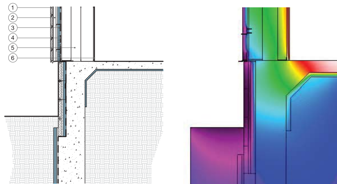
As-Built Condition
